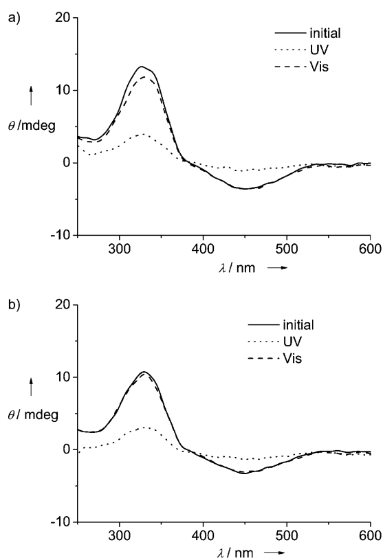
Figure 6. Circular dichroism spectra of an aqueous solution of Azo-C1-N + /α-CD (a) and diluted sol of PEG/α-CD/Azo-C1-N + (b), before (—) and after (•••••) UV and visible-light (----) irradiation. C(\text{Azo-C1-N}^+) = 1 \times 10^{-3} M, n(\alpha\text{-CD}):n(\text{Azo-C1-N}^+) = 1:1 .
