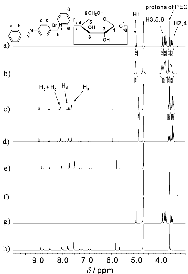
Figure 2. ^1\text{H} NMR spectra of a) PEG/ \alpha -CD solution, b) PEG/ \alpha -CD hydrogel, c) PEG/ \alpha -CD/Azo-C1-N ^+ , d) \alpha -CD/Azo-C1-N ^+ , e) Azo-C1-N ^+ , f) PEG, g) \alpha -CD, and h) PEG/Azo-C1-N ^+ solutions in \text{D}_2\text{O} .
