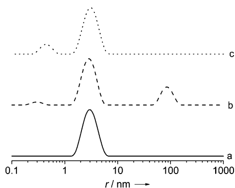
Figure 3. DLS results for PEG (—), PEG/ \alpha -CD (----), and PEG/ \alpha -CD/Azo-C1-N ^+ (.....) aqueous solutions.
